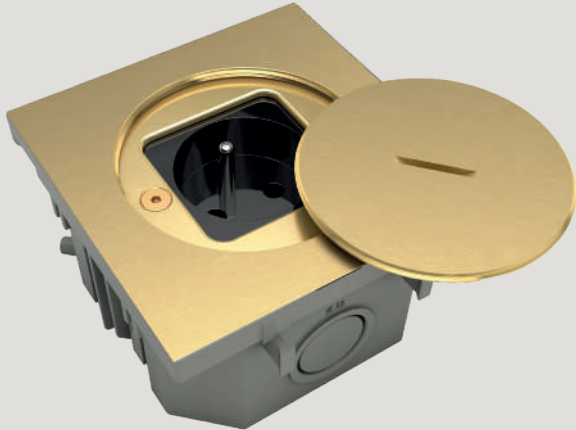
PRISE 2P+T FRANCO-BELGE - BFL102/1
